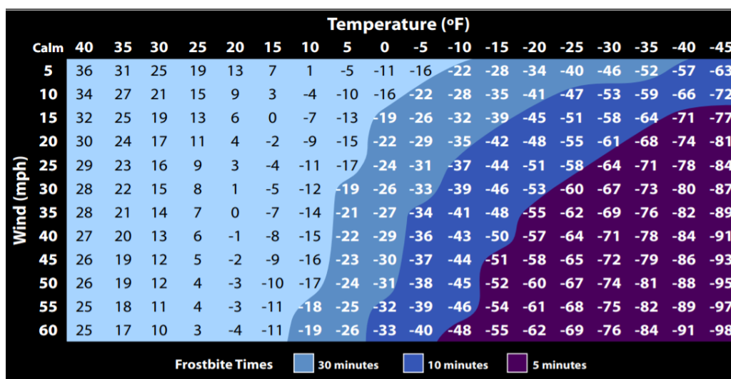
Figure 1. Wind Chill Chart 1
